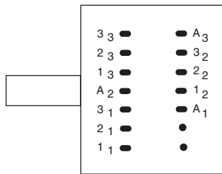
3 POLES 2-3 POSITIONS
