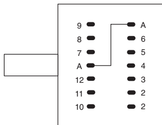
1 POLE 2-12 POSITIONS
